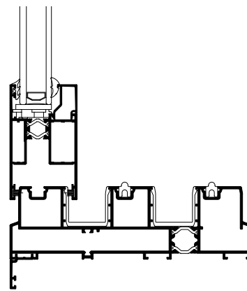
trirail
