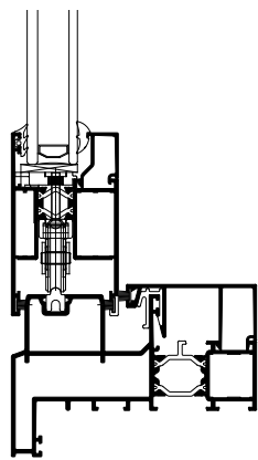
monorail
